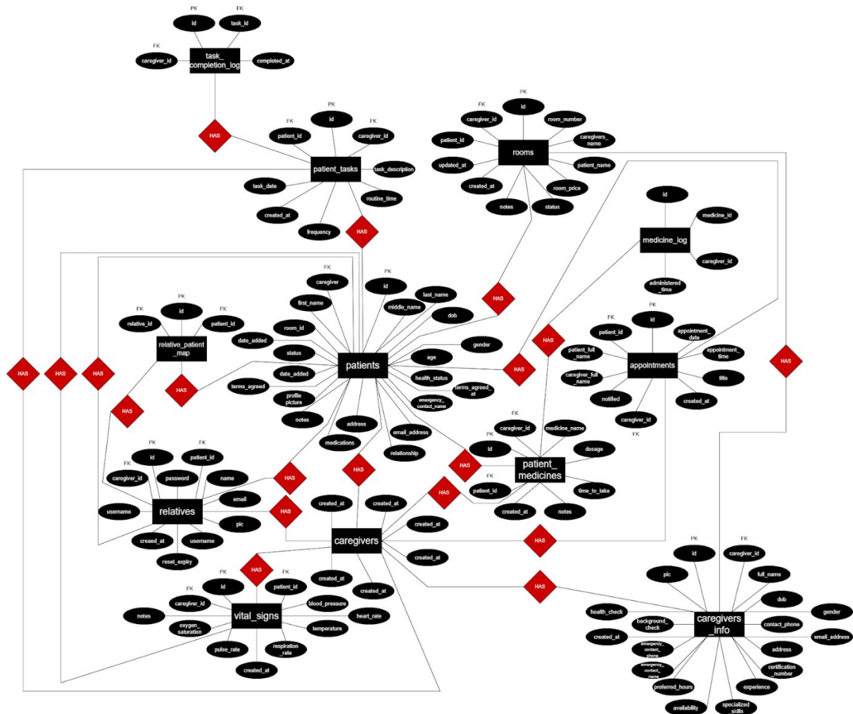
Figure 4. Entity Relation Diagram
