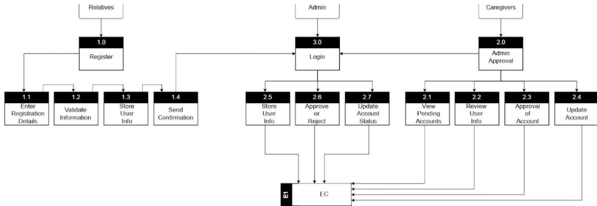
Figure 3. Level 2 Data Flow Diagram
