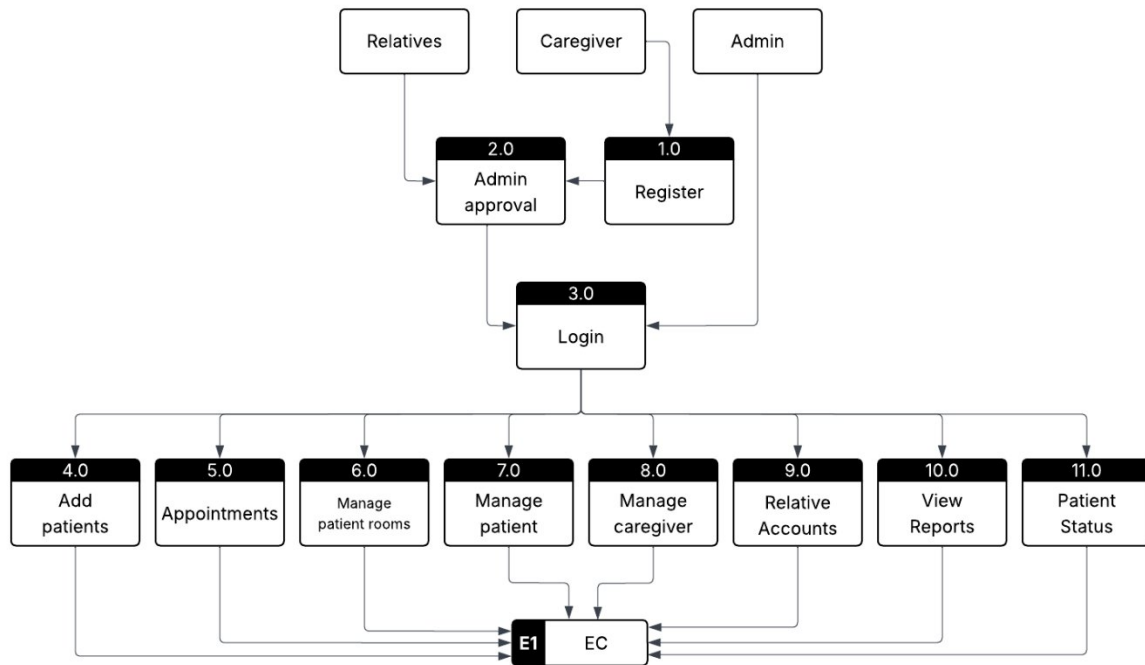
Figure . Level 1 Data Flow Diagram
